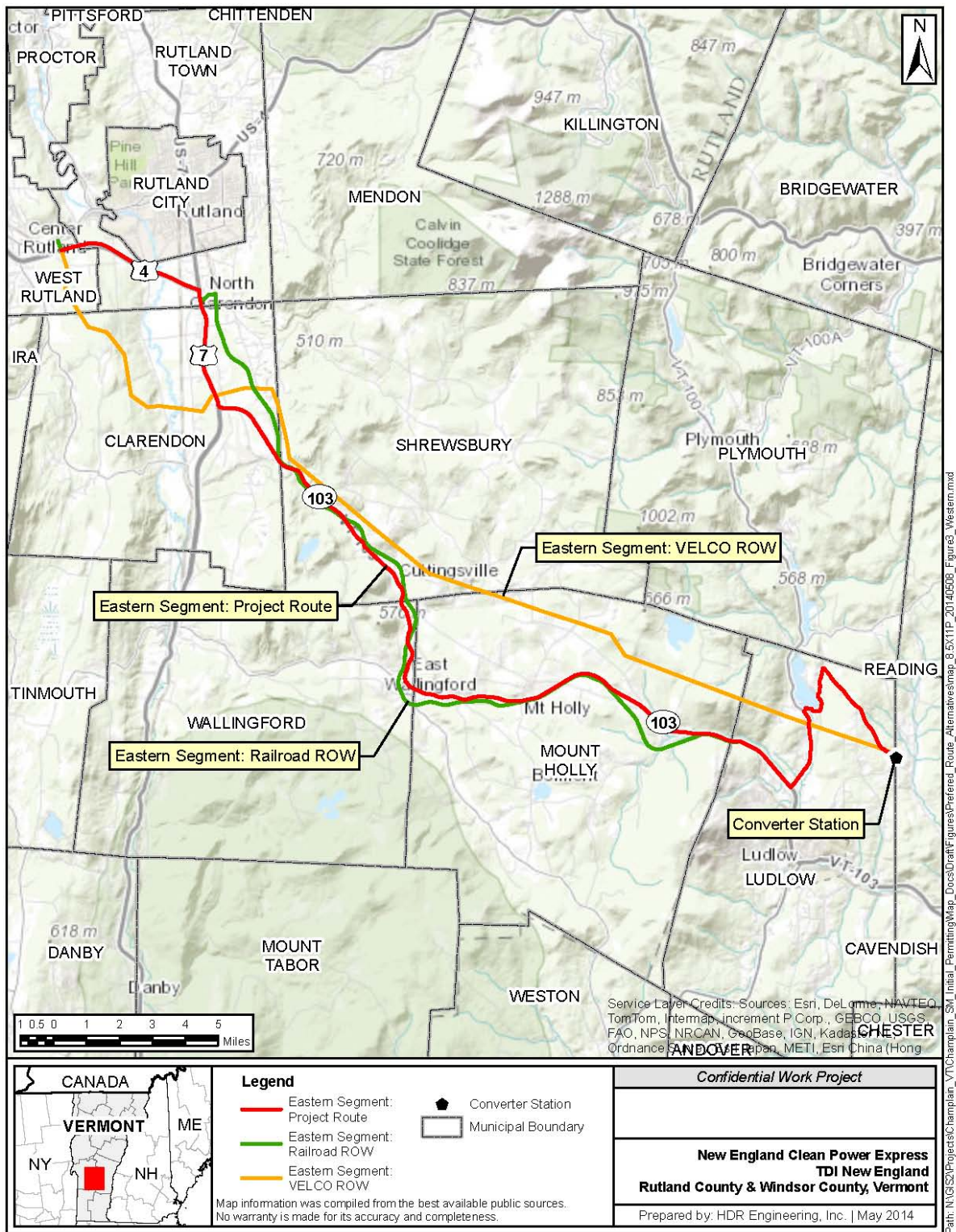
FIGURE 4-4 EASTERN SECTION ALTERNATIVES
