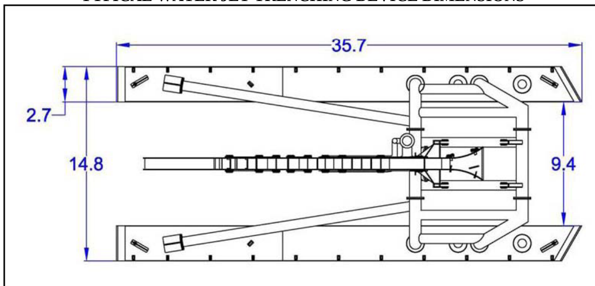
FIGURE 2-14 TYPICAL WATER JET TRENCHING DEVICE DIMENSIONS
